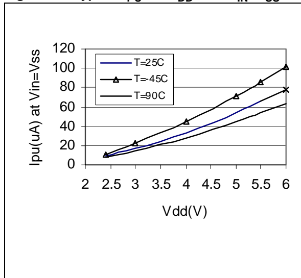
Figure 78. Typical V_{IL}
