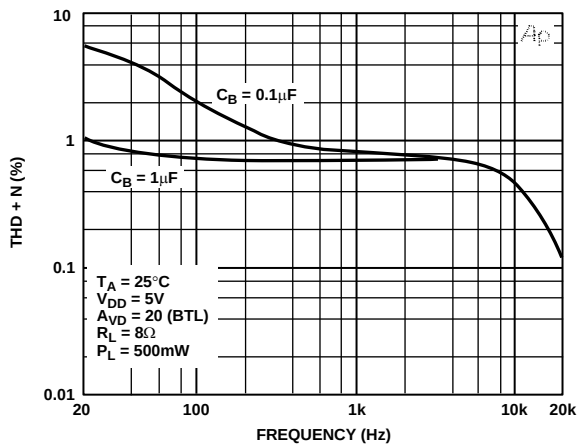
Figure 6. THD + N vs. Frequency
