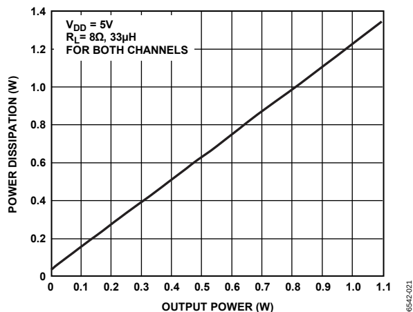
Figure 21. Power Dissipation vs. Output Power at V_{DD} = 5V , R_L = 8\Omega
