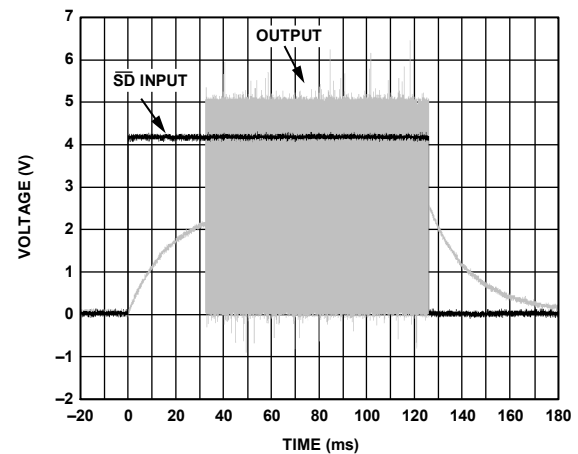
Figure 31. Turn-Off Response
