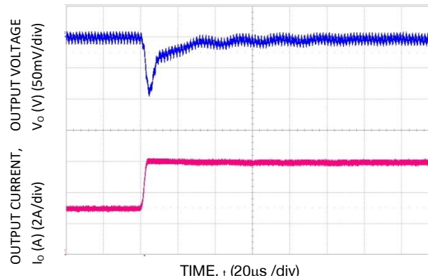
Figure 24. Transient Response to Dynamic Load Change from 50% to 100% at 12 Vin, C_{out} = 2 \times 47 \mu F , C_{Tune} = 2200 \text{ pF} , R_{Tune} = 261 \Omega . V_o = 5.0 \text{ V}
