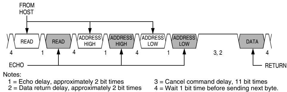
Figure 17-15. Read Transaction
