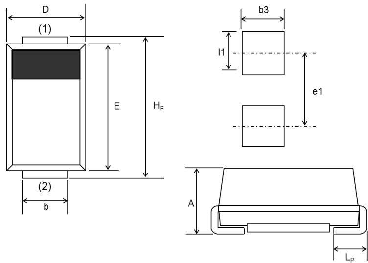
DO-214AC(SMA), (FVDS)
