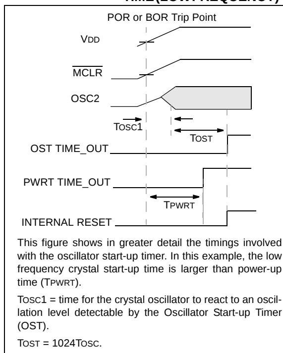
FIGURE 5-4: OSCILLATOR START-UP TIME (LOW FREQUENCY)
