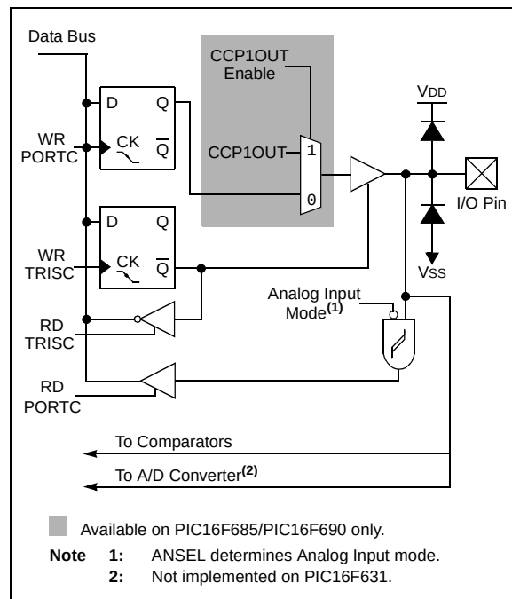
FIGURE 4-12: BLOCK DIAGRAM OF RC2 AND RC3
