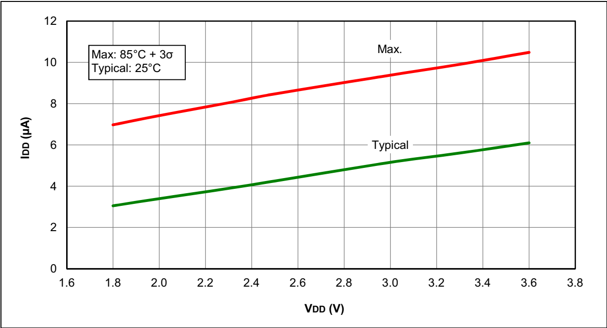
FIGURE 29-13: I DD , LFINTOSC, F osc = 31 kHz, PIC16LF1503 ONLY
