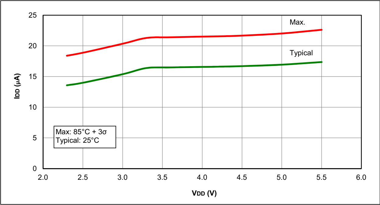
FIGURE 29-14: I DD , LFINTOSC, F osc = 31 kHz, PIC16F1503 ONLY
