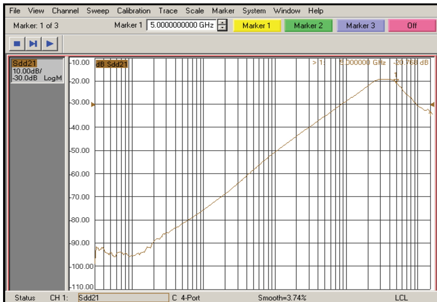
Fig 5. Off Isolation
