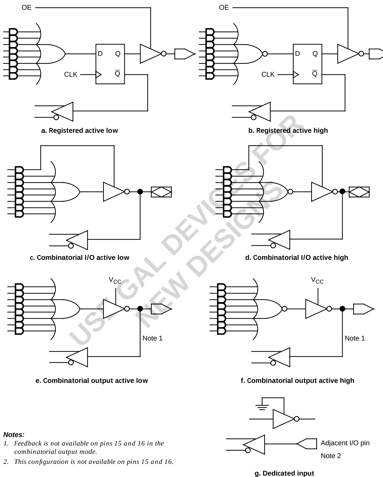
Figure 2. Macrocell Configurations
