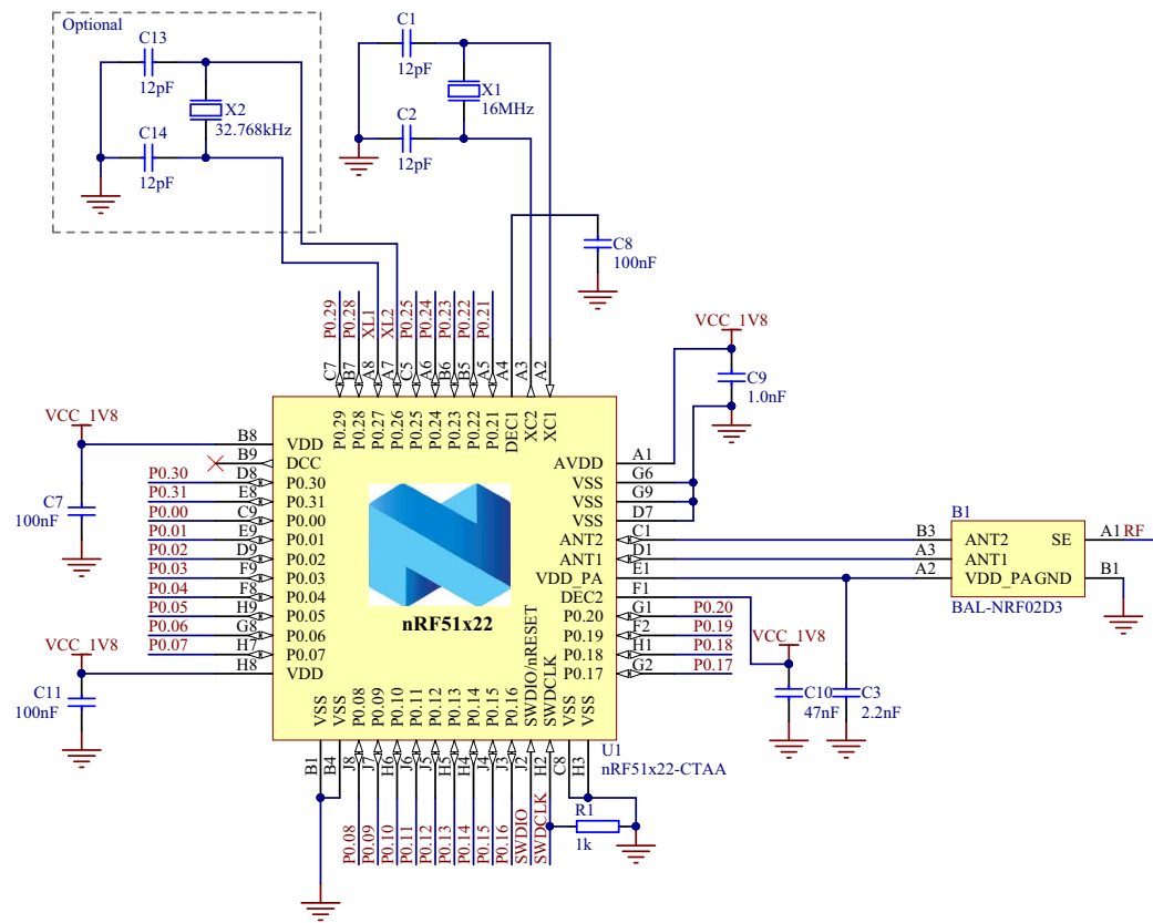
Figure 43 CTAA WLCSP with low voltage mode setup
