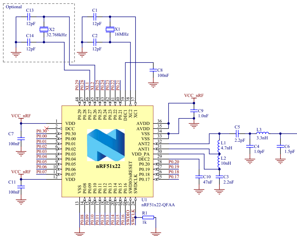
Figure 24 QFAA QFN48 with internal LDO setup
