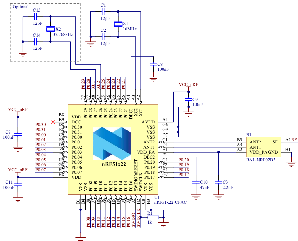
Figure 39 CFAC WLCSP with internal LDO setup
