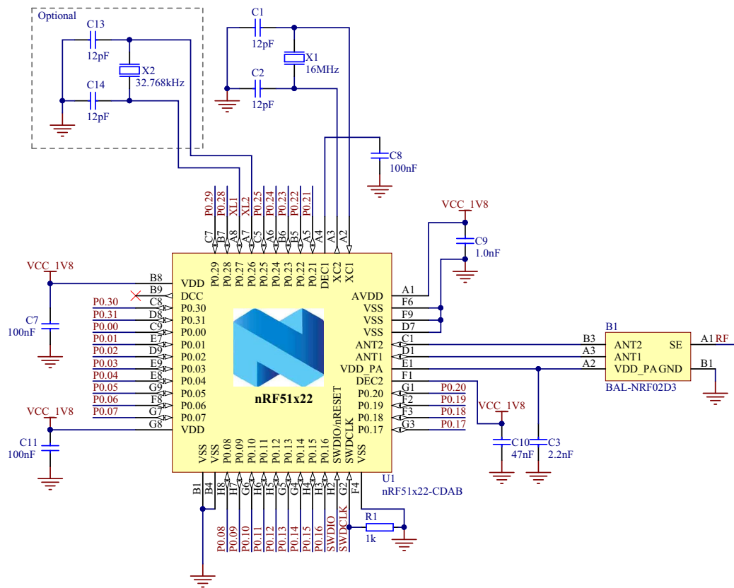
Figure 34 CDAB WLCSP with low voltage mode setup
