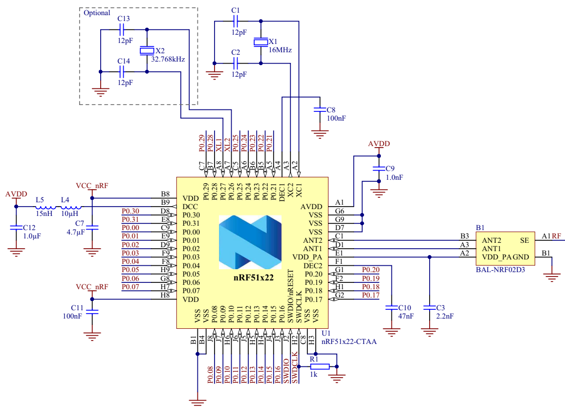
Figure 44 CTAA WLCSP with DC/DC converter setup
