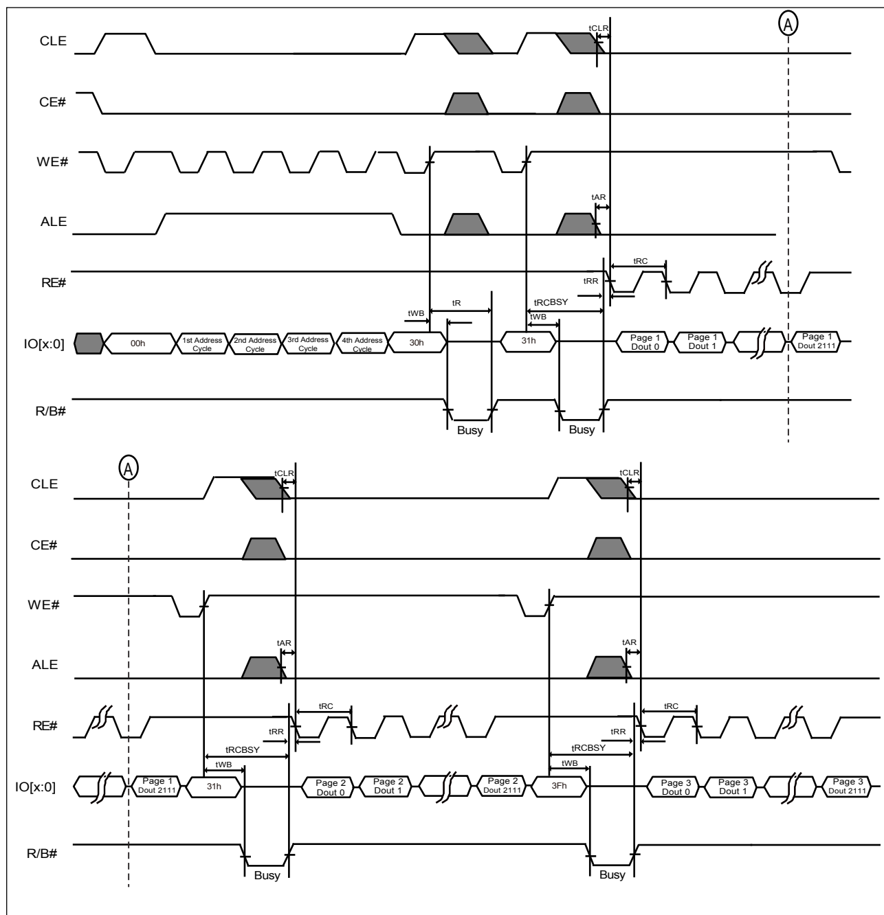
Figure 11-1. AC Waveforms for Cache Read Sequential
