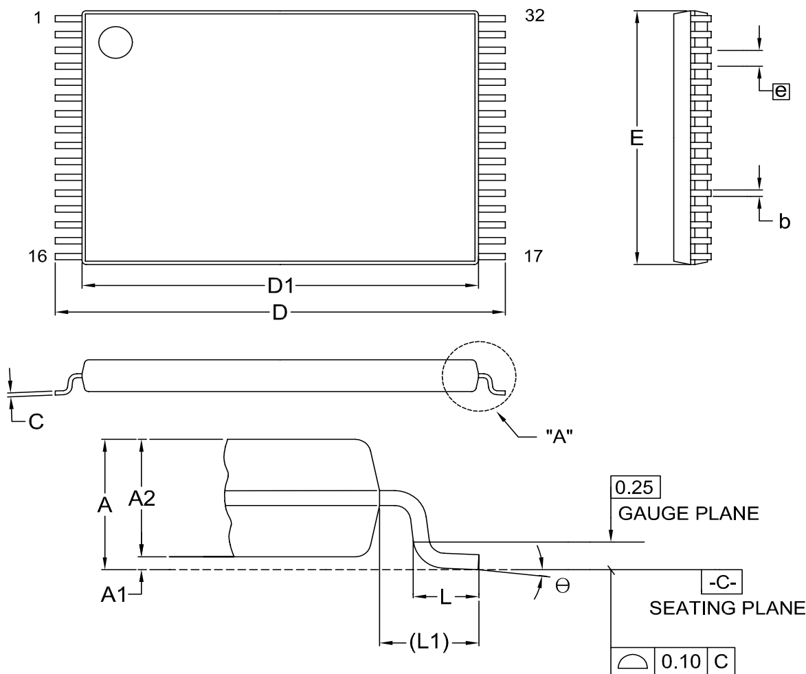
DETAIL "A"
