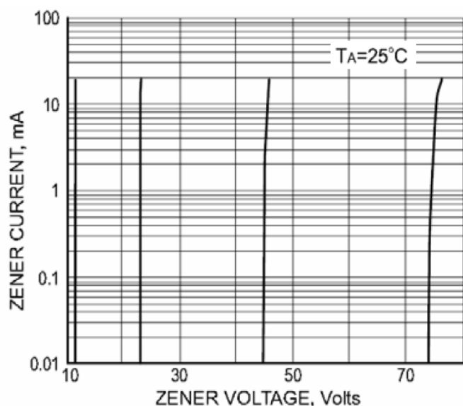
Fig.3 Typical Zener Breakdown Characteristics
