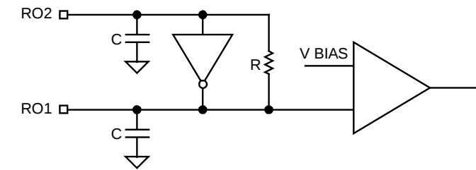
Figure 5. Reference Oscillator Circuit
