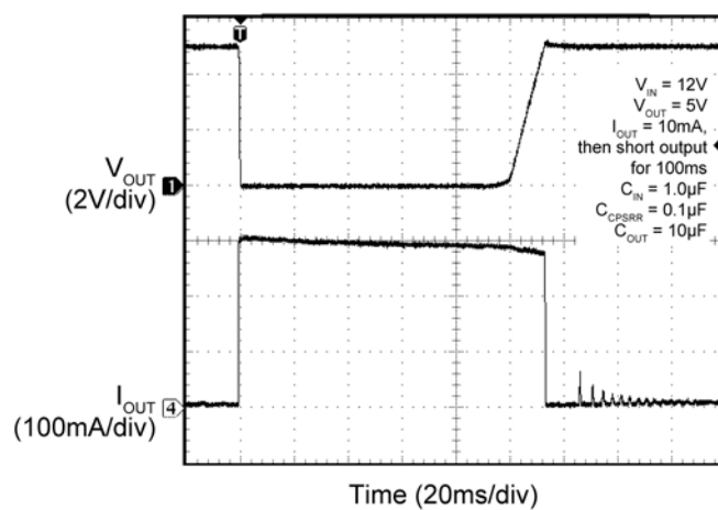
Current Limit
