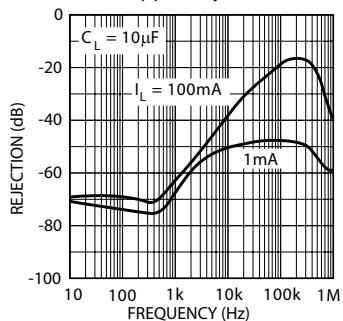
Ripple Rejection
