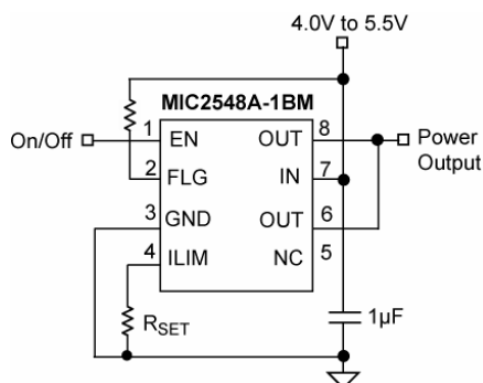
Figure 3. Supply Bypassing
