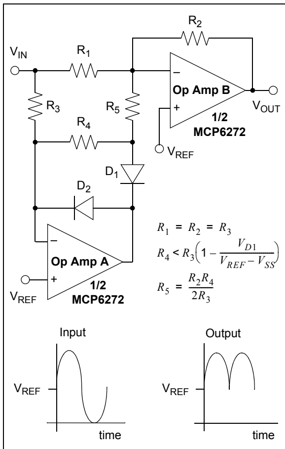
FIGURE 4-8: Active Full-wave Rectifier.
