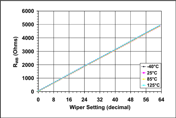
FIGURE 2-25: 5 kΩ – R_{WB} (Ω) vs. Wiper Setting and Ambient Temperature.
