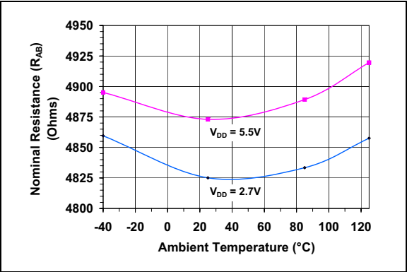
FIGURE 2-24: 5 kΩ – Nominal Resistance (Ω) vs. Ambient Temperature and V_{DD} .
