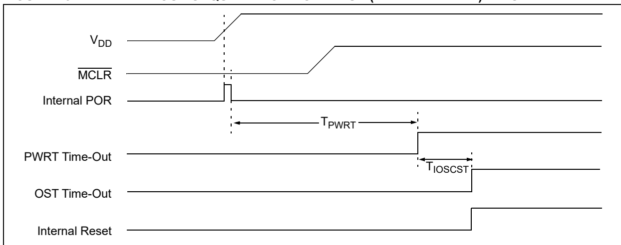
FIGURE 13-4: TIME-OUT SEQUENCE ON POWER-UP (DELAYED \overline{\text{MCLR}} ): CASE 1
