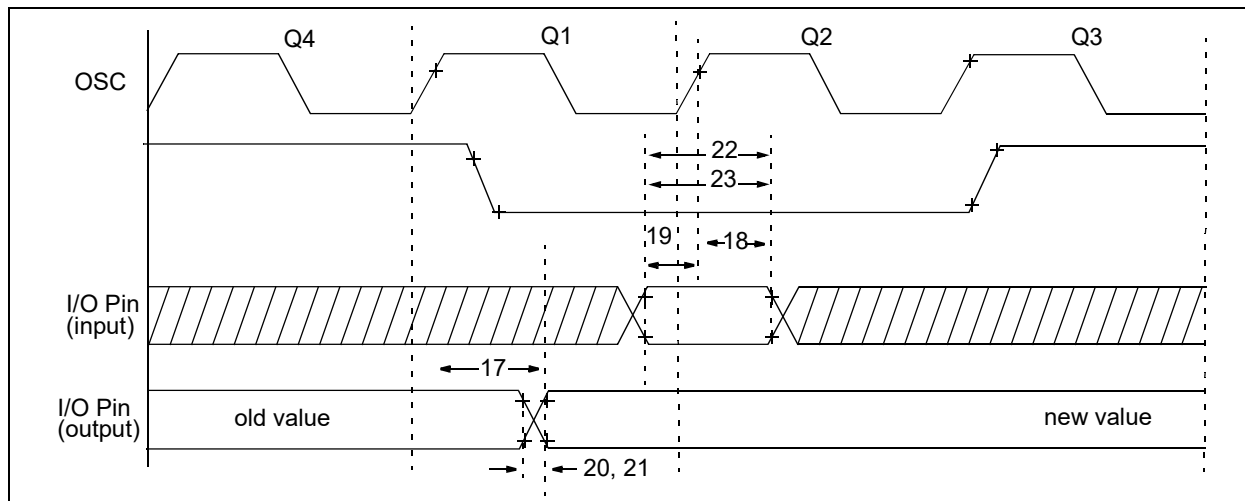
FIGURE 5-3: I/O TIMING
