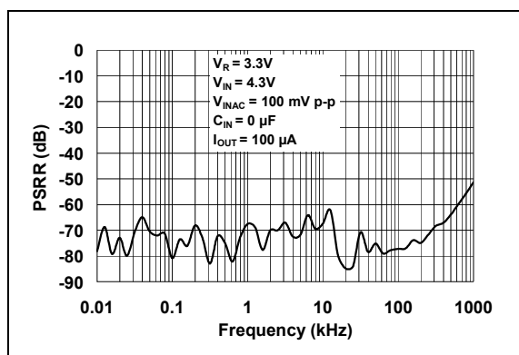
FIGURE 2-24: PSRR vs. Frequency.
