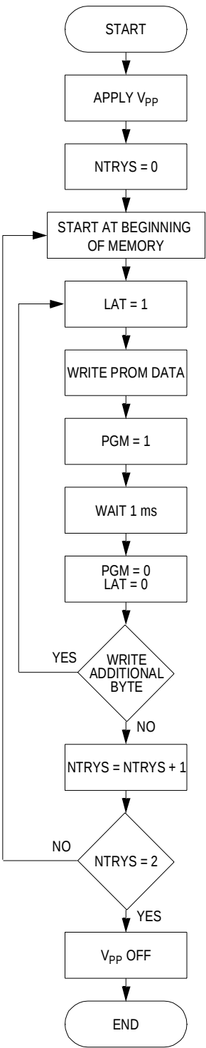
Figure 9-1. EPROM/OTPRO Programming Flowchart
