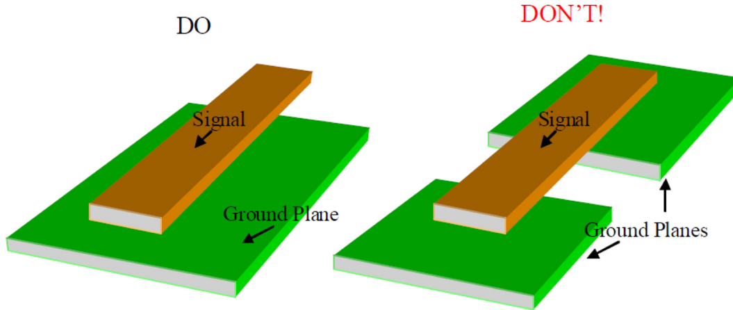
Figure 29. Recommended shielding for critical signals
