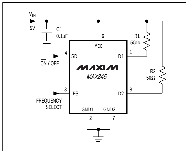
Figure 1. Test Circuit
