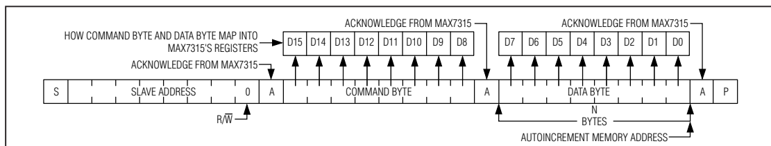
Figure 9. n Data Bytes Received
