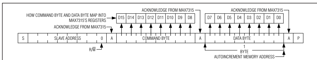
Figure 8. Command and Single Data Byte Received
