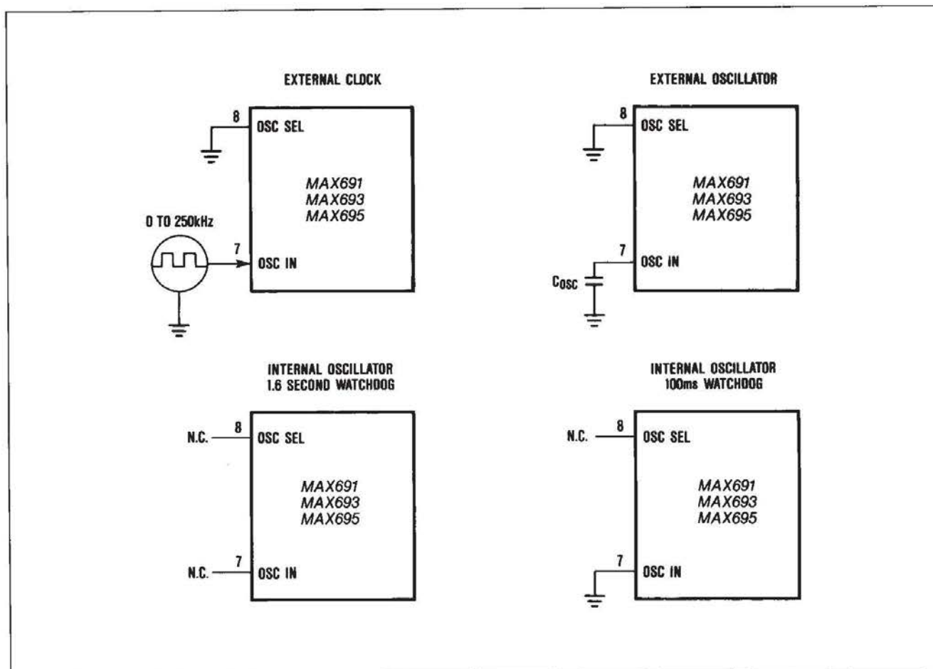
Figure 8. Oscillator Circuits
