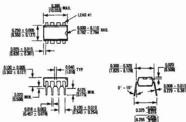
8 Lead Plastic DIP (PA)
