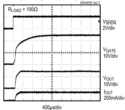
STARTUP WAVEFORM FROM SHUTDOWN (C IN = 10μF, C OUT = 10μF)
