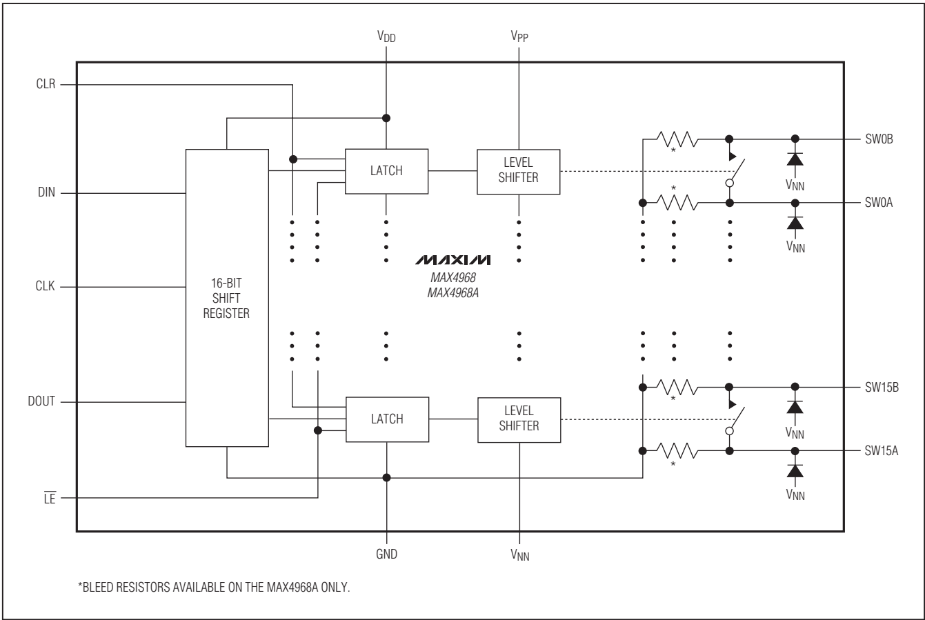
Functional Diagram
