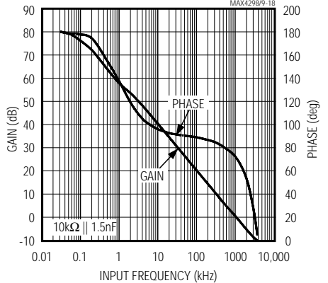
DRIVER OUT OPEN-LOOP FREQUENCY RESPONSE
