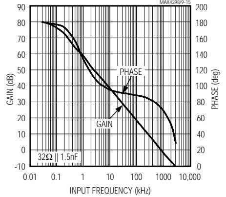
DRIVER OUT OPEN-LOOP FREQUENCY RESPONSE
