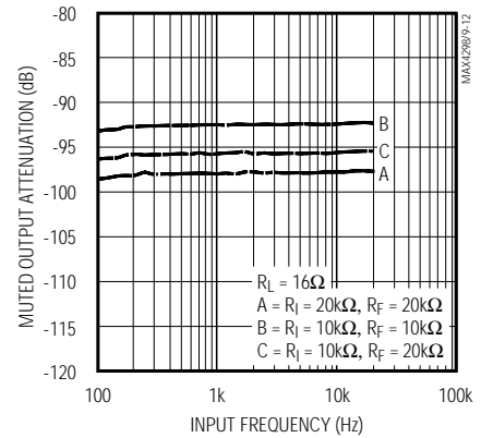
DRIVER OUT MUTED OUTPUT ATTENUATION vs. INPUT FREQUENCY
