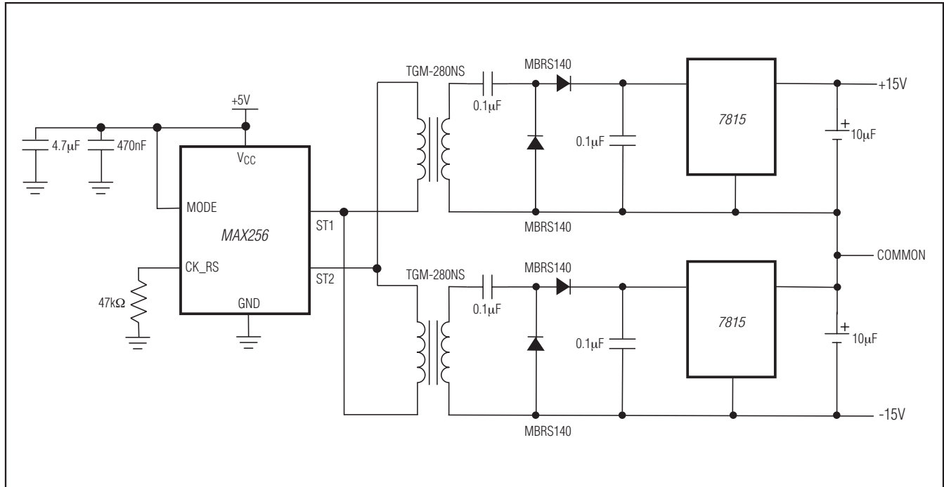
Figure 5. +5V to Isolated Regulated \pm 15V
