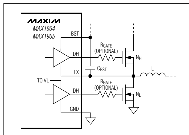
Figure 5. Reducing the Switching EMI
