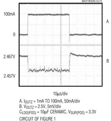
POSITIVE LINEAR REGULATOR LOAD TRANSIENT ( Q_{LDO} = 2N3905 )
