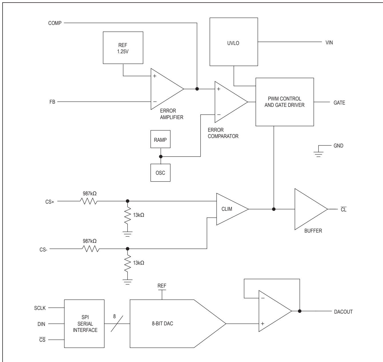
Figure 1. Functional Diagram
