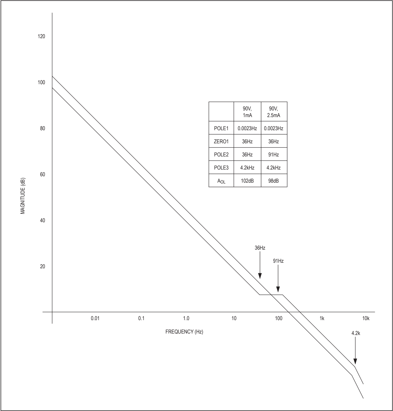
Figure 6. Loop Response
