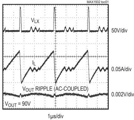
SWITCHING WAVEFORMS
