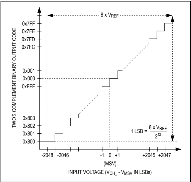
Figure 14. ±10V Bipolar Transfer Function
