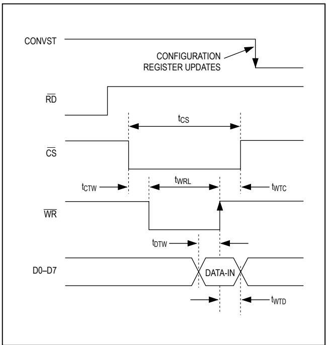
Figure 6. Write Timing
