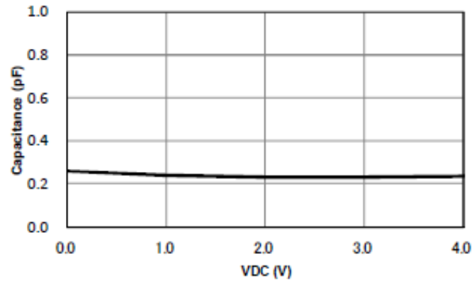
Voltage—Capacitance Characteristic
