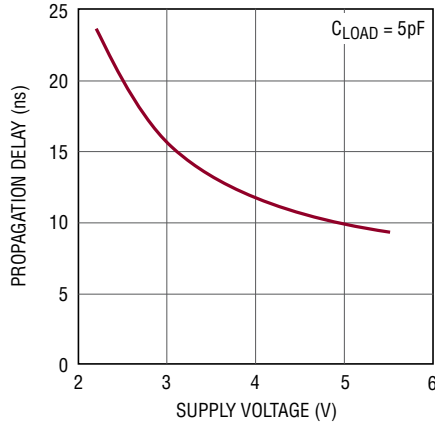
Input Propagation Delay ( t_{PD} ) vs Supply Voltage
