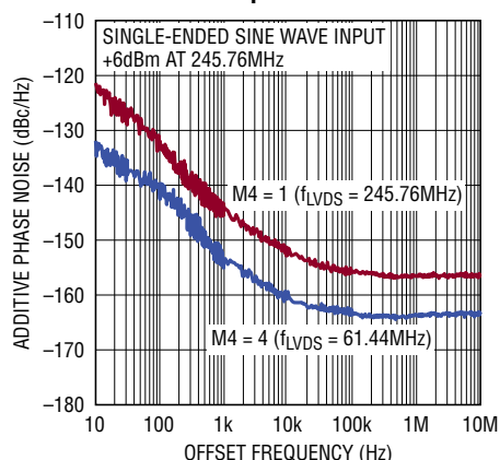
LVDS Additive Phase Noise with 245.76MHz Input
