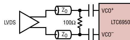
AC-COUPLED LVDS
