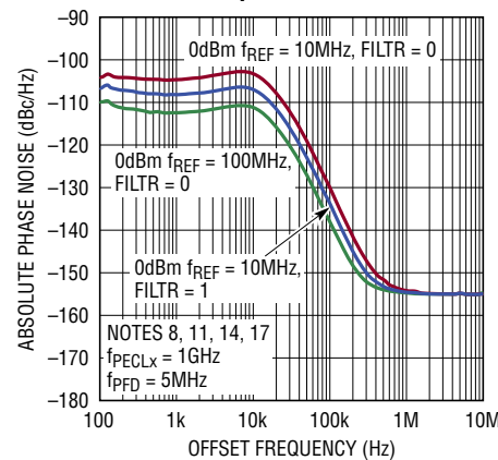
PECLx Closed-Loop Phase Noise 10MHz vs 100MHz Sine Wave Reference Input
