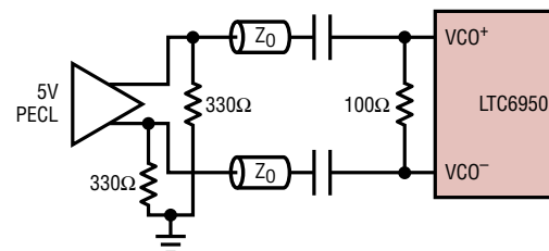
AC-COUPLED 5V PECL
