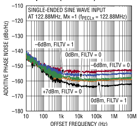
PECLx Additive Phase Noise vs Amplitude (IBIASx = 1)
