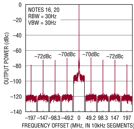
PECLx Spurious Response f_{VCO} = 1.2288GHz , f_{PFD} = 49.152MHz
