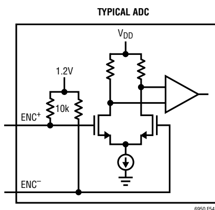
Figure 51. Simplified Sample Clock Input Circuit
