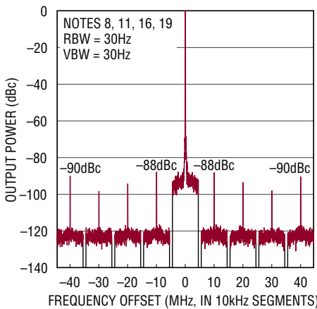
PECLx Spurious Response f_{VCO} = 1GHz , f_{PFD} = 10MHz
