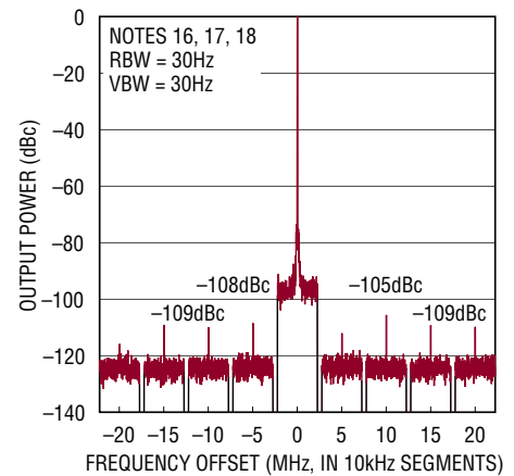
PECLx Spurious Response f_{VCO} = 125MHz , f_{PFD} = 5MHz
