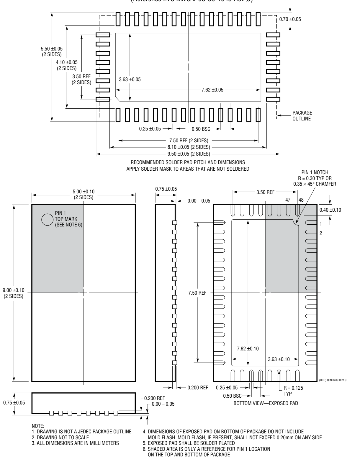
UHH Package 48-Lead Plastic QFN (5mm × 9mm) (Reference LTC DWG # 05-08-1845 Rev 0)
