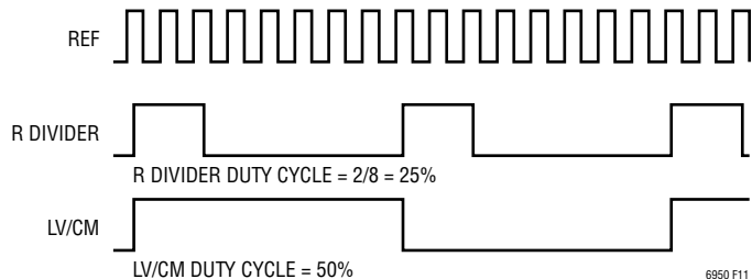
Figure 11. LV/CM Duty Cycle (R = 8, M4 = 2)
