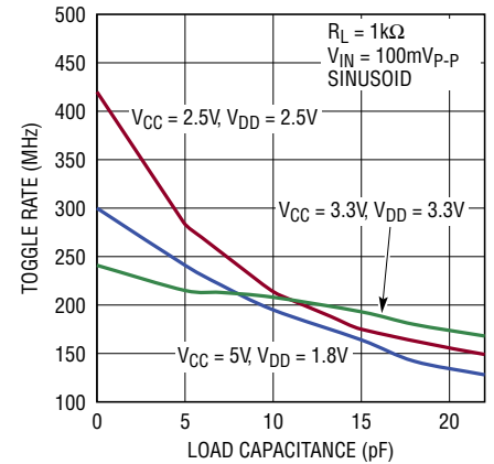
Toggle Rate vs Capacitive Load, (LTC6752/LTC6752-1/LTC6752-2/ LTC6752-4)
