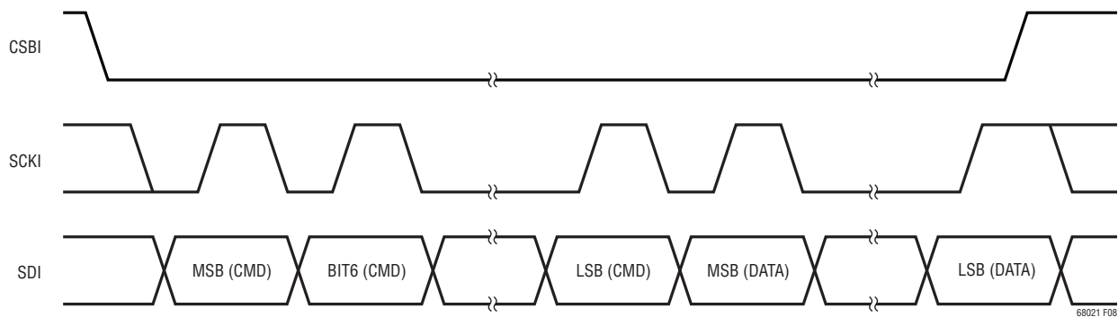
Figure 8. Transmission Format (Write)
