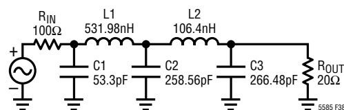
Figure 38. Final Design Schematic
