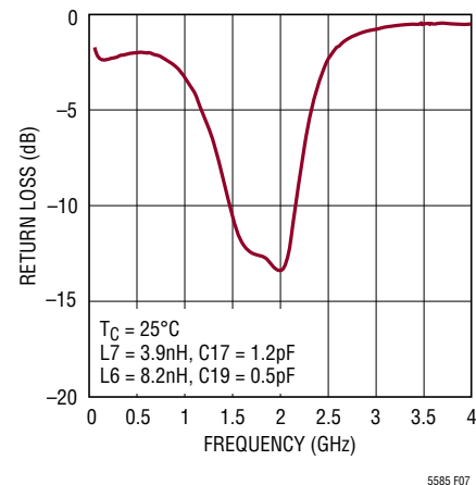
Figure 7. RF Input Return Loss for Wideband Match
