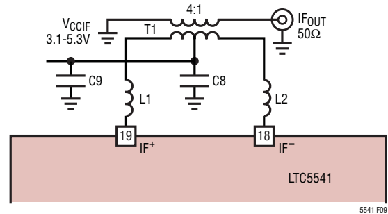
Figure 9. IF Output with Lowpass Matching
