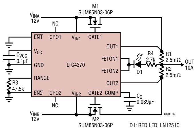
Figure 6. Current Sharing 12V Supplies
