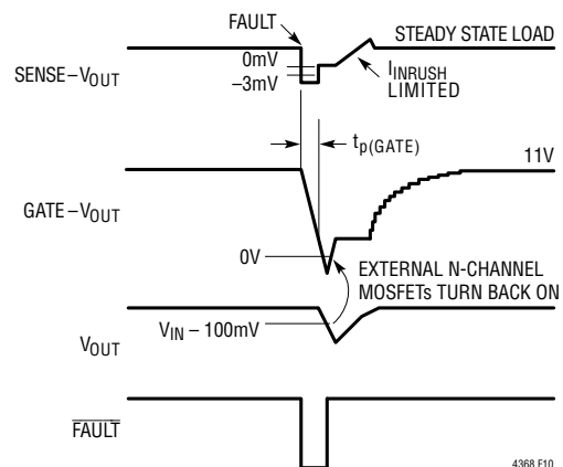
Figure 10. Reverse Overcurrent Fault: \text{SENSE} - V_{\text{OUT}} < -3\text{mV} (LTC4368-2)
