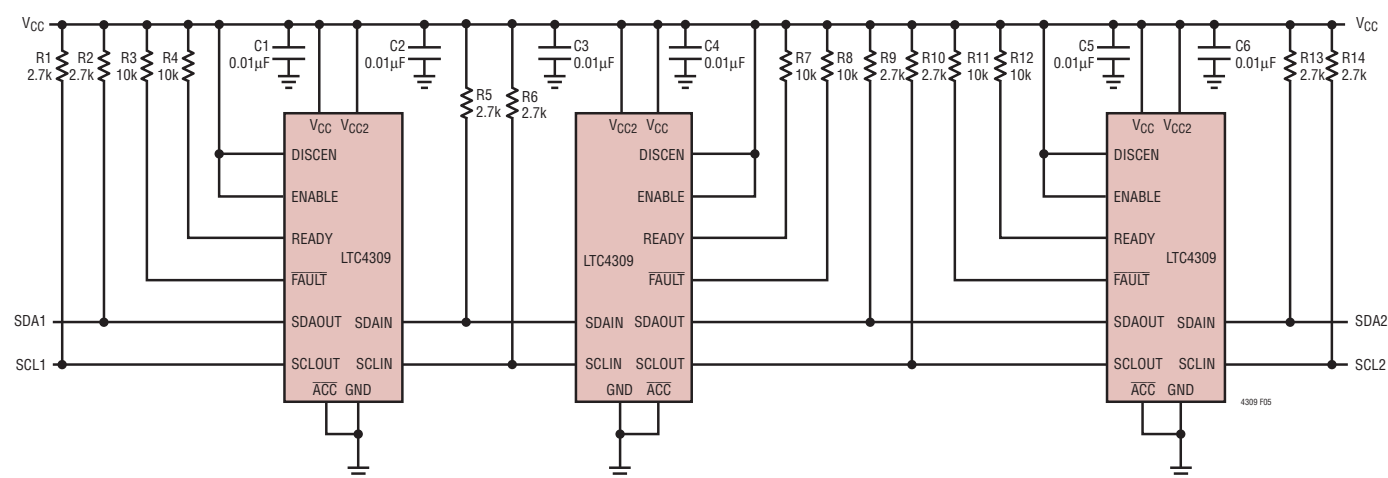
Figure 7. The LTC4309 in a Repeater Application. The LTC4309's Low Offset Allows Cascading of Multiple Devices.
