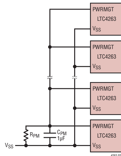
Figure 5. PWRMGT Pin Connections
