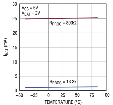
Trickle Charge Current vs Temperature (4065L and 4065L-4.1)
