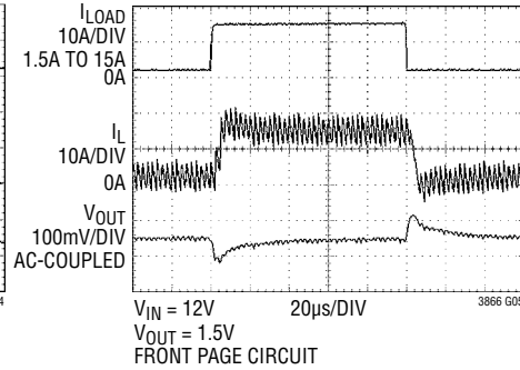
Load Step (Continuous Conduction Mode)
