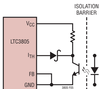
Figure 5. Circuit for Isolated Feedback
